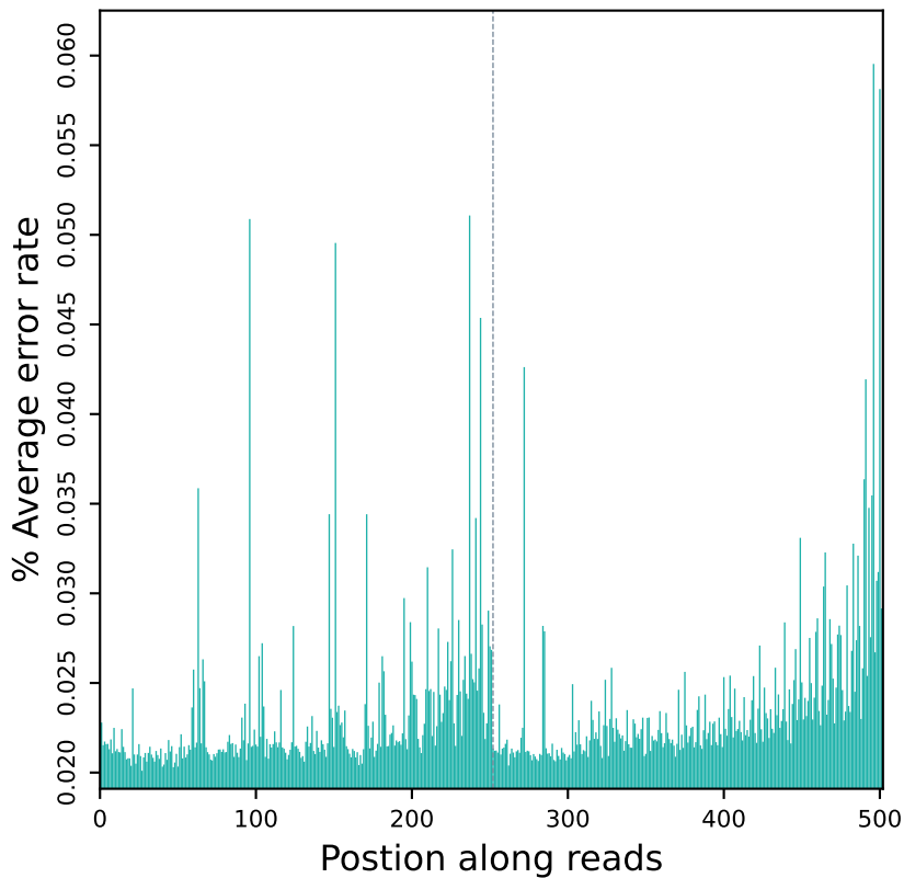
Error rate distribution along reads (R10920)
